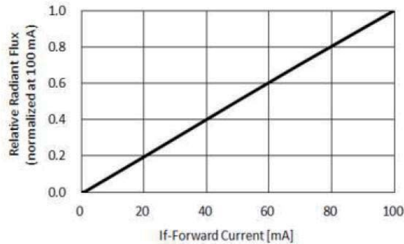
Fig.1 – Relative Radiant Flux vs. Forward Current
