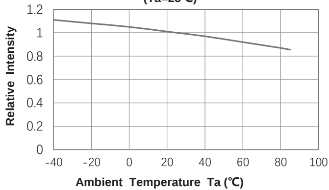
Relative Intensity VS. Ambient Temperature (Ta=25°C)
