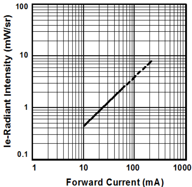
Fig.4 Radiant Intensity vs. Forward Current
