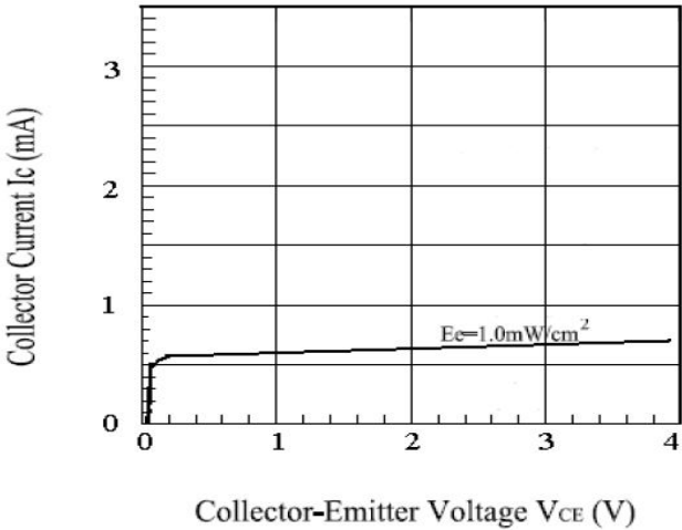
Fig.3 Collector Current vs Collector-Emitter Voltage
