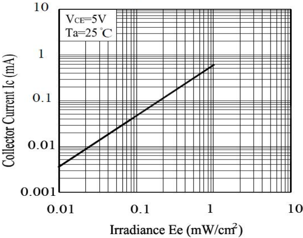
Fig.2 Collector Current vs irradiance
