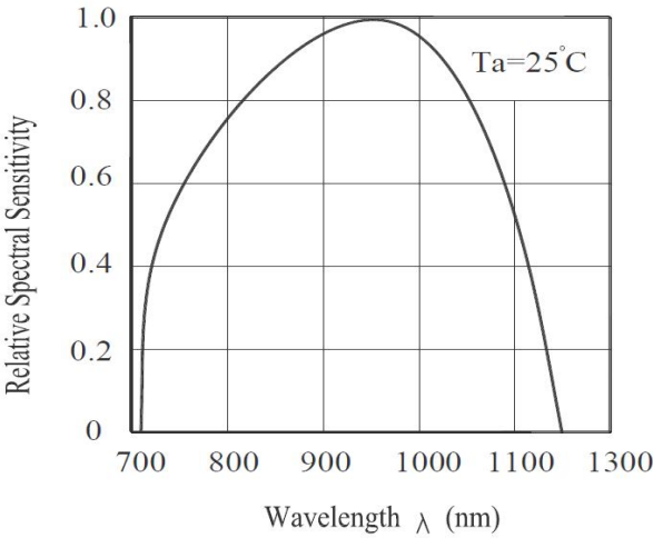
Fig.1 Spectral Sensitivity
