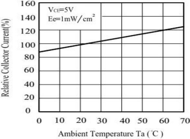
Fig.4-Relative Collector Current vs. Ambient temperature
