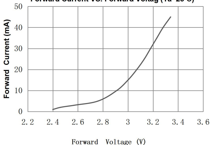
Forward Current VS. Forward Voltag (Ta=25°C)
