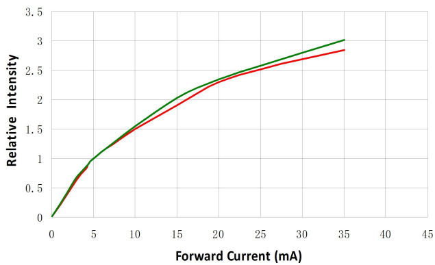
Relative Intensity VS. Forward Current ( T_a=25^\circ\text{C} )
