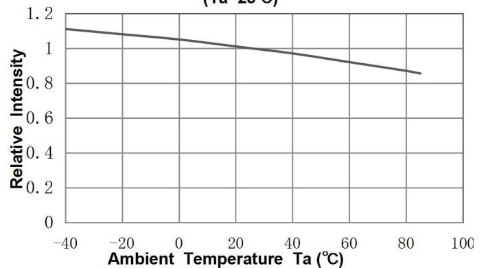
Relative Intensity VS. Ambient Temperature (Ta=25°C)
